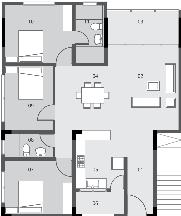
Typical 3 BHK unit plan with indicative furniture layout
